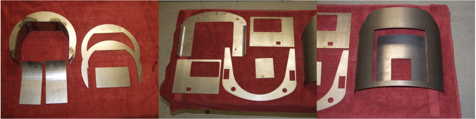
Smokebox Feedwater Heater Piping Ditch Parts
