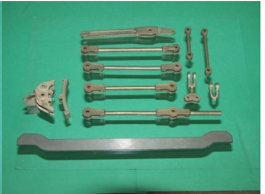
Tender Truck Brake Parts
